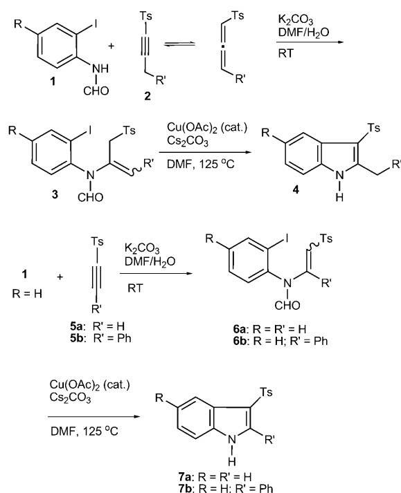
Scheme 1. Synthesis of indoles from o -iodoanilines and acetylenic sulfones 2 and 5 .
