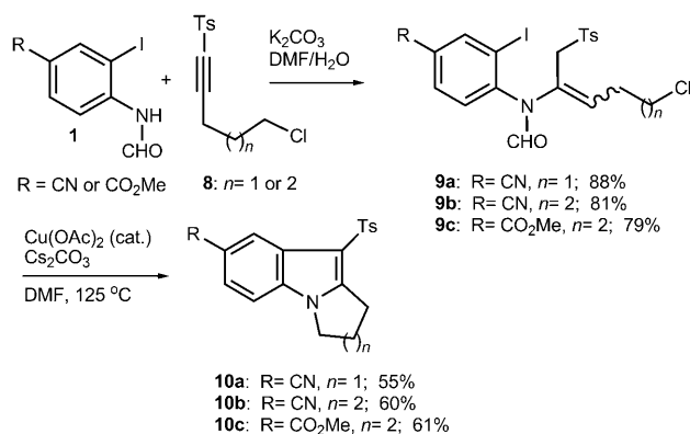
Scheme 2. Tandem cyclizations with acetylenic sulfones 8 .
