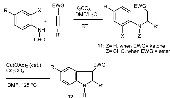
Scheme 3. Synthesis of indoles from o -iodoanilines and ynoates or ynone.
