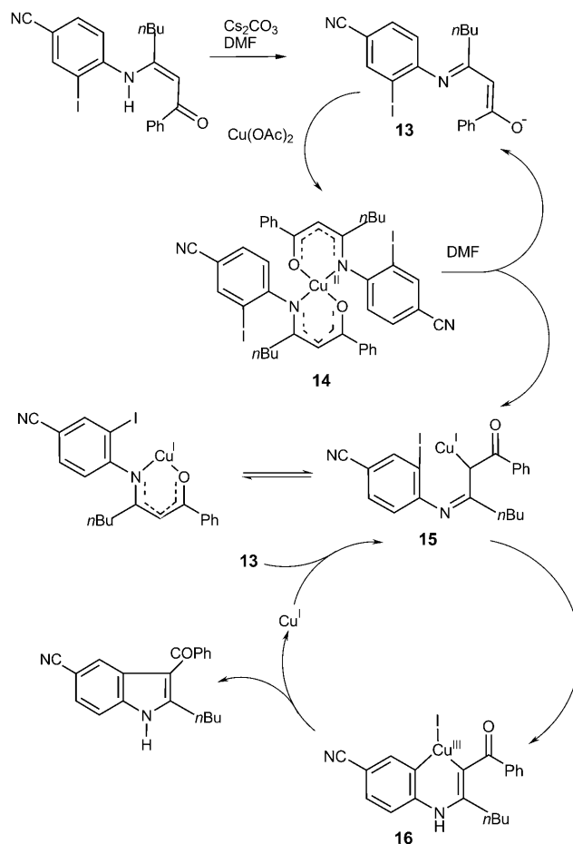
Scheme 4. Cu(OAc) 2 -mediated enaminone cyclization.
