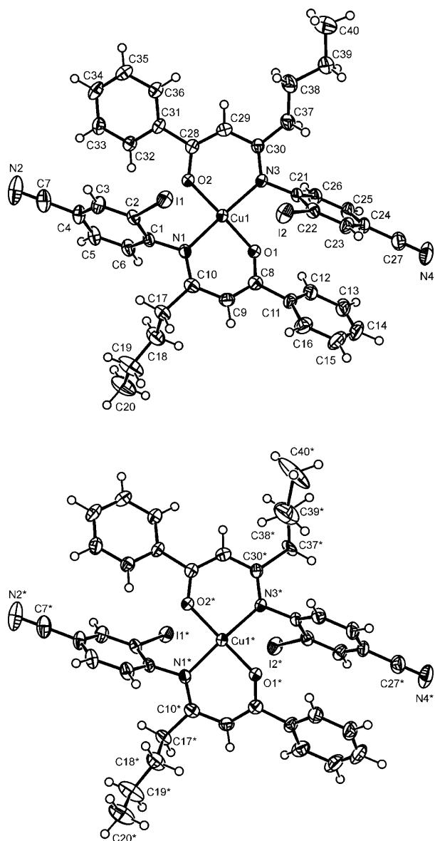
Figure 1. ORTEP diagrams (50% probability) of the two conformations of 14 (see Supporting Information for details). [16]
